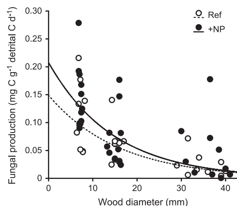
FIG. 3. The relationship between wood diameter and wood-associated fungal production. Since fungal production depends on temperature, the raw production data from August 2004 and June 2005 only (stream and incubation temperatures of 15°C) were used for this graph. By the linear regression model (not shown), R^2 = 0.42 and P < 0.001 for the reference stream and R^2 = 0.33 and P = 0.001 for the nutrient-enriched stream. By the negative exponential model, y = 0.149e^{-0.063x} , R^2 = 0.60 , and P < 0.001 for the reference stream and y = 0.207e^{-0.068x} , R^2 = 0.43 , and P < 0.001 for the nutrient-enriched stream. d -1 , per day; Ref, reference stream; +NP, nutrient-enriched stream.
