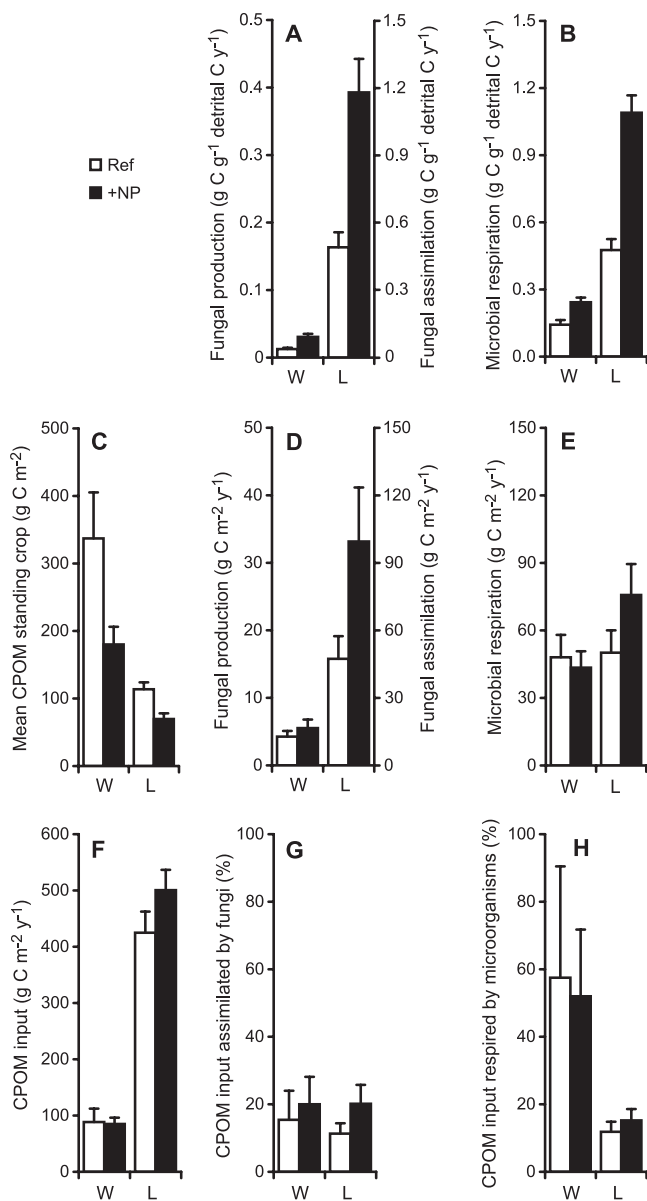
FIG. 4. Annual ecosystem-level estimates of microbial activity associated with and microbial importance in the decomposition of small wood and leaf litter in the reference and the nutrient-enriched streams for July 2004 to July 2005. (A) Annual fungal production and assimilation (fungal growth efficiency of 0.33 was used to calculate assimilation) (45). (B) Annual microbial respiration (respiratory quotient of 0.95 was assumed). (C) Mean small wood and leaf litter standing crop. (D) Annual fungal production and assimilation per stream bottom area. (E) Annual microbial respiration on an areal basis. (F) Annual small wood and leaf litter input. (G and H) Estimates of CPOM input assimilated by fungi and lost through microbial respiration. Means and upper 95% CL are shown since values were estimated by bootstrapping, except in panels C and F, where SE are shown. Note that panels A and B answer the question of how fast submerged detrital carbon is used by microorganisms, while panels G and H show what proportion of annual riparian subsidies is utilized by microorganisms. L, leaves; W, wood; Ref, reference stream; +NP, nutrient-enriched stream.
