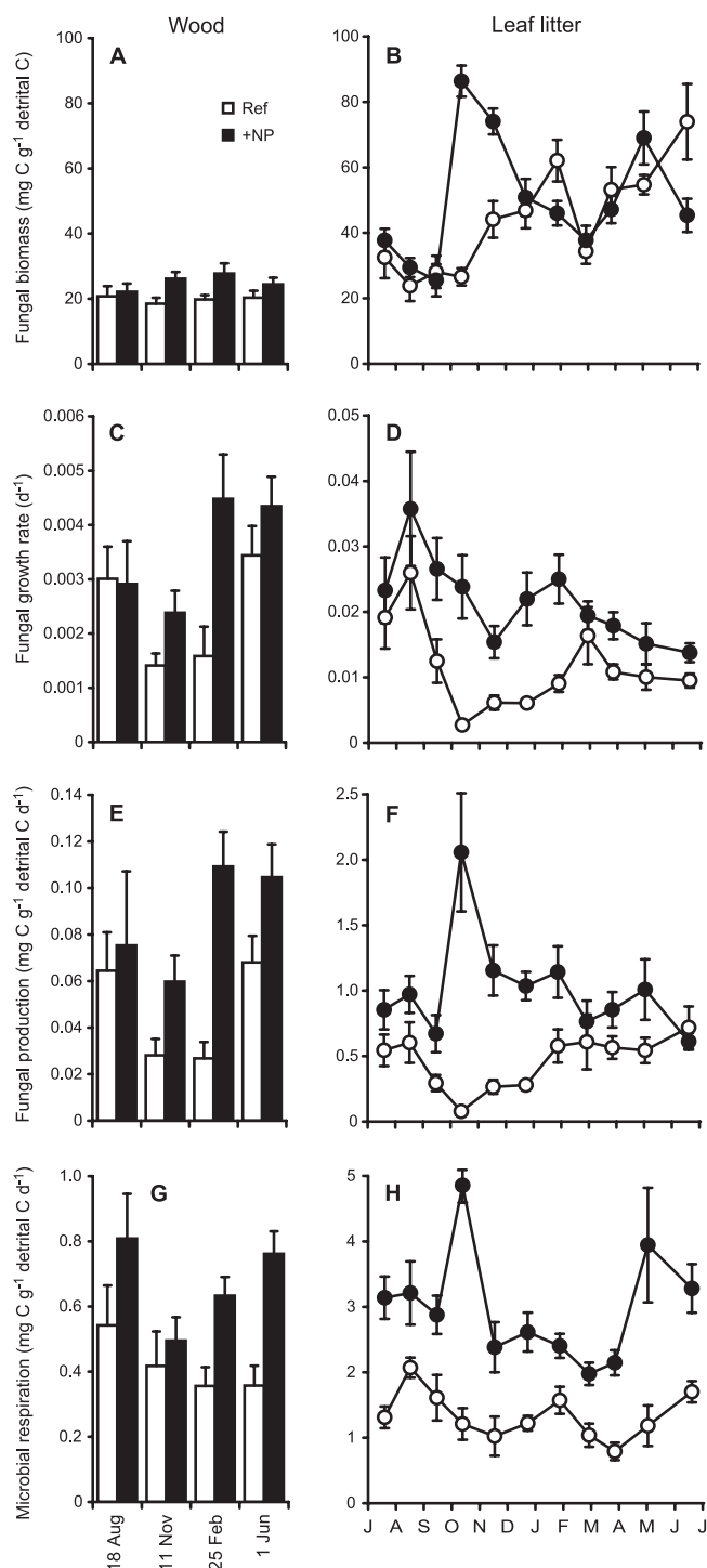
FIG. 1. Fungal biomass (A and B), instantaneous fungal growth rate (C and D), daily fungal production (E and F), and microbial respiration (G and H) associated with decomposing small wood and leaf litter in the reference and the nutrient-enriched streams during the 1-year study period. Data are per unit of detrital carbon. Error bars indicate 1 SE ( n = 15 for wood and n = 5 for leaves). d^{-1} , per day; Ref, reference stream; +NP, nutrient-enriched stream.
