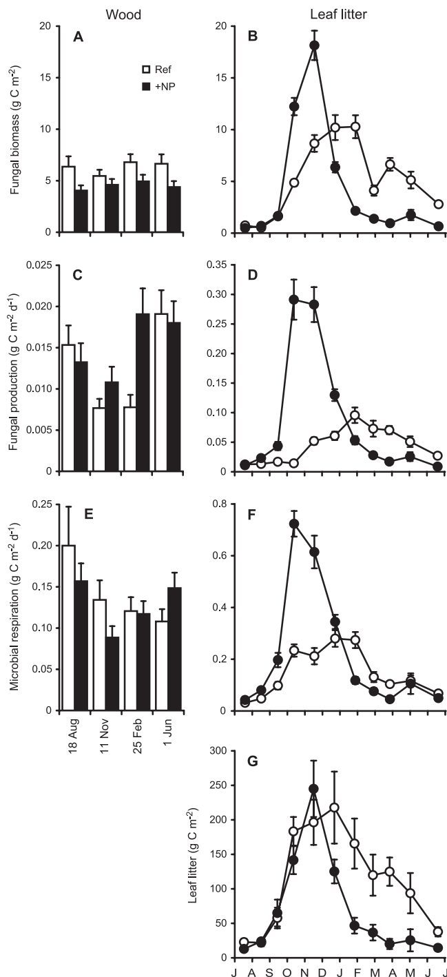
FIG. 2. Seasonal changes in fungal biomass (A and B), production (C and D), and microbial respiration (E and F) per unit of stream bottom area for small wood and leaf litter in the reference and the nutrient-enriched stream. Highly seasonal dynamic of leaf litter standing crop is given in panel G, to aid in interpreting leaf-associated fungal and respiration data. Small wood standing crop is given on Fig. 4C. Error bars indicate 1 SE. d -1 , per day; Ref, reference stream; +NP, nutrient-enriched stream.
