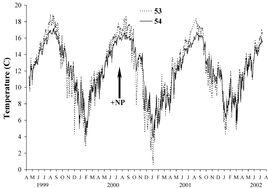
FIG. 1. Average daily water temperatures of stream 53 and 54 during the study.
